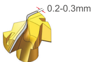
a) 磨损极限 Wear Limit
