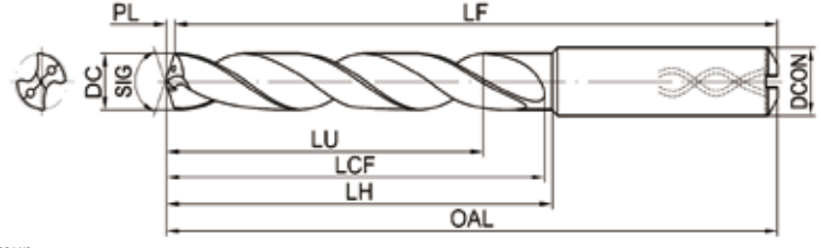
Internal coolant design
