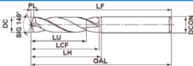
External coolant design
